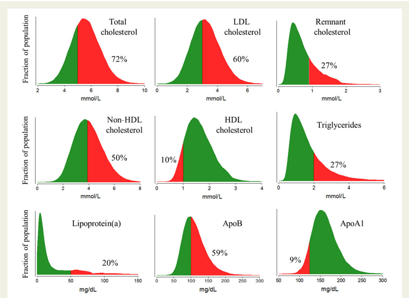
Figure 8 Proportion of non-fasting individuals in the general population with flagged abnormal concentrations in laboratory reports using desirable concentration cut-points as shown in Table 5. Of all participants, 12% were receiving statins. Figure designed by Prof. B.G. Nordestgaard and Dr A. Langsted based on unpublished data on 92 285 non-fasting individuals from the Copenhagen General Population Study recruited in 2003 through 2014.
